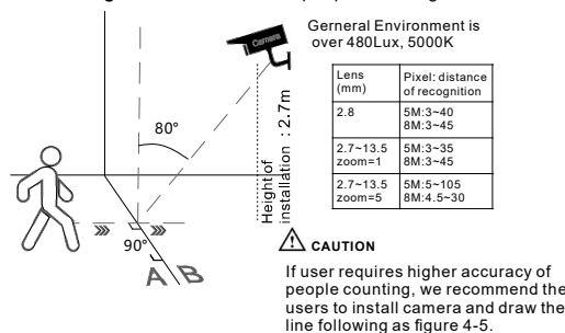
Figure 4-4 Installation of people counting
