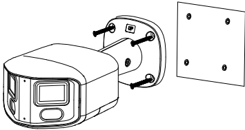
Figure 3-2 Installing camera
